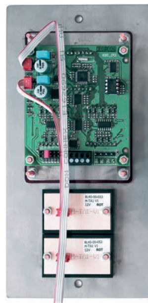
Back view Shaft module
